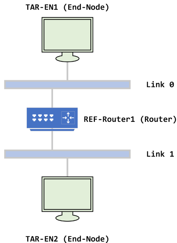
FIGURE 1 – END-NODE V. END-NODE: TRANSPORT AND TUNNEL MODE
