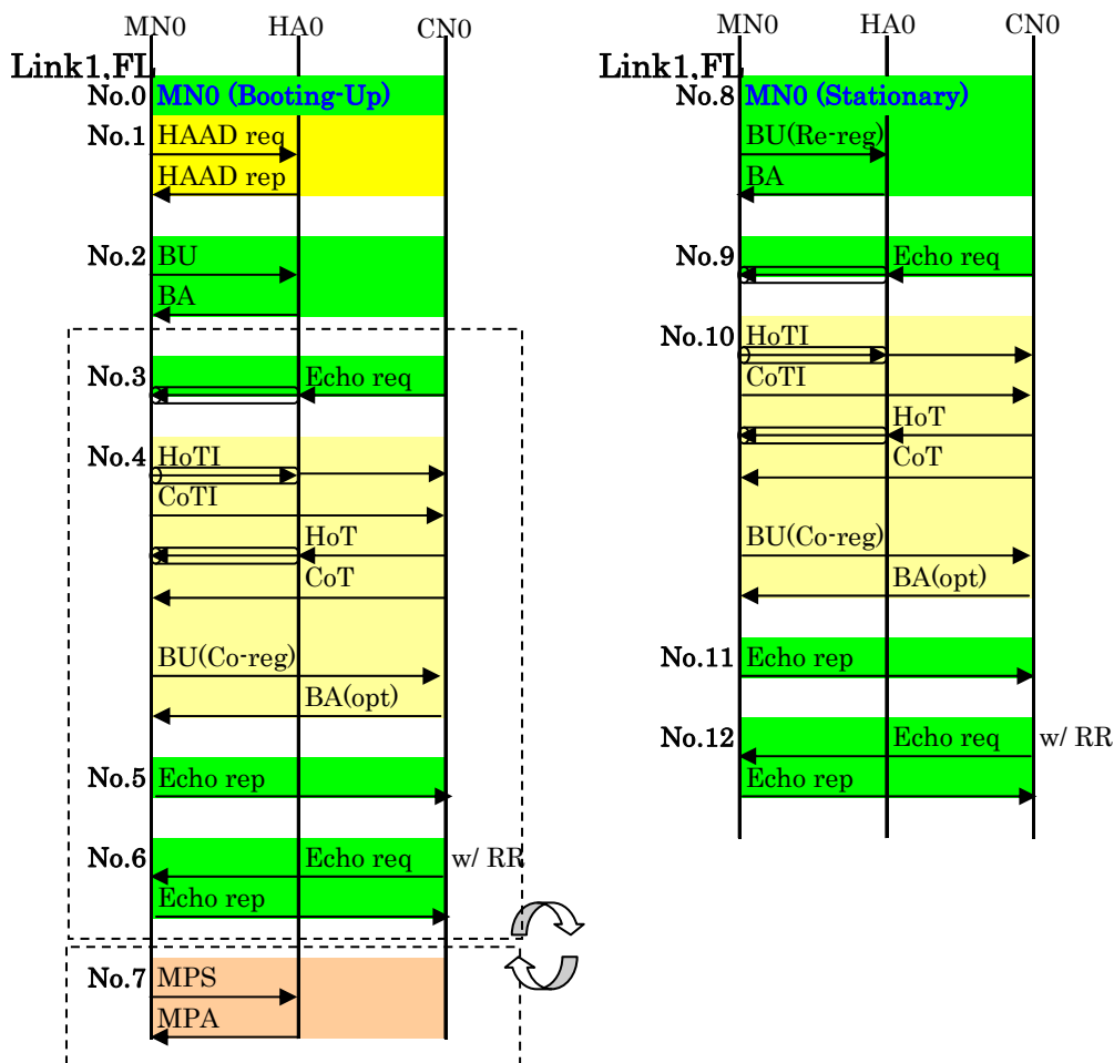
Sequence of Interoperability Test Scenario(1/3)
